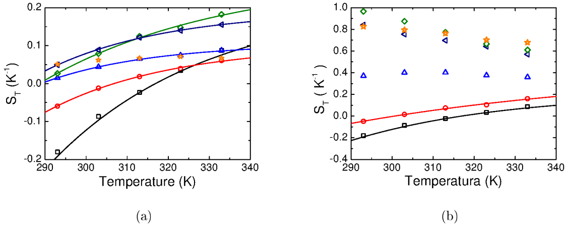
Figure 4: Soret coefficient of the nanoparticles (particles concentration of 0.5 mg/mL) as function of temperature for some concentrations of the added salts TMAOH (a) and TBAOH (b): 0 mMol/L (black squares), 0.1 mMol/L (red circles), 0.5 mMol/L (blue triangles), 1 mMol/L (olive diamonds), 2 mMol/L (navy triangles) and 20 mMol/L (orange stars). The solid lines in the corresponding colors are the best fit curves with Iacopini's equation S_T(T) = S_T^\infty (1 - e^{(T^*-T)/T_0}) .
